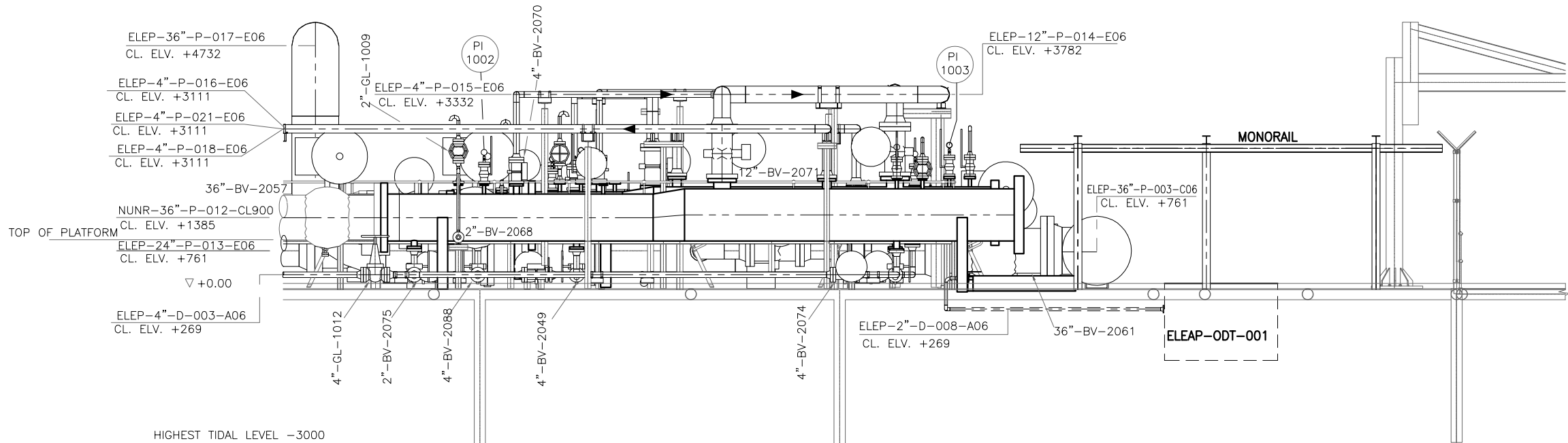
B 01 SECTION B-B
